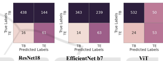
Figure 6: Comparative Analysis of the confusion metrics obtained from the encoders experimented with, as tabulated in Table 5. The values are on the testing dataset, which consists of 582 samples belonging to the 'TB' class and 77 samples belonging to the 'TE' class.
