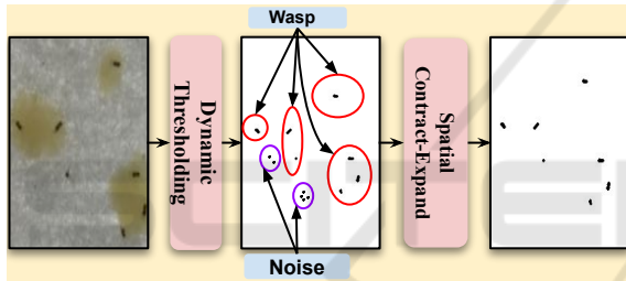
Figure 3: ROI Extraction: First, dynamic thresholding is performed to dissociate the foreground ( i.e. , wasps) from the background ( i.e. , the arena and eggs) from the original image. Next, a spatial contract-expand operation is performed in binary image to remove the additional noises.
