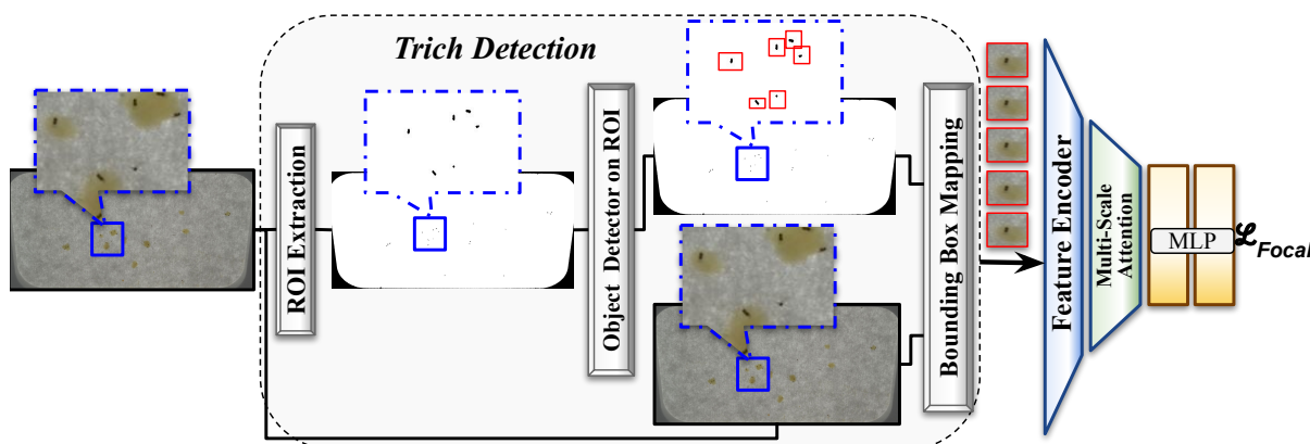
Figure 2: Proposed Method: First, pre-processing is done on the input HR images, after which it is broken into patches and passed through a pre-trained YOLOX detector. The detections obtained are then passed through a pre-trained ViT encoder, followed by the proposed MSGA module, and finally a classification head, to obtain the class probability matrix.
