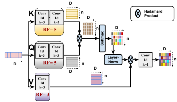
Figure 4: Proposed Multi-Scale Attention Module: It generates a multi-scale attentive feature map by projecting the input feature map to different convolutional receptive fields ( i.e. RF=3,5). Here RF=5 projection encodes the coarse-level contextual feature, whereas RF=3 projection provides the fine-grained cue. Hence an attentive feature map generated from such a coarse-fine encoding ensures to capture discriminability in spatial cues across species categories.
