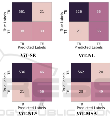
Figure 5: Comparative Analysis of the confusion metrics obtained from experiments with various popular attentive enhancements and the proposed attention module, results of which have been tabulated in Table 2. The values are on the testing dataset, which consists of 582 samples belonging to the 'TB' class and 77 samples belonging to the 'TE' class.
