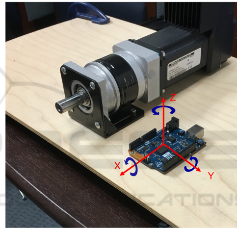
Figure 4: Orientations of sensors on Arduino relative to the motor.
