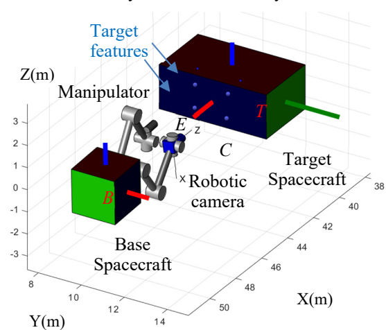
Figure 1: On-orbit servicing scenario.
