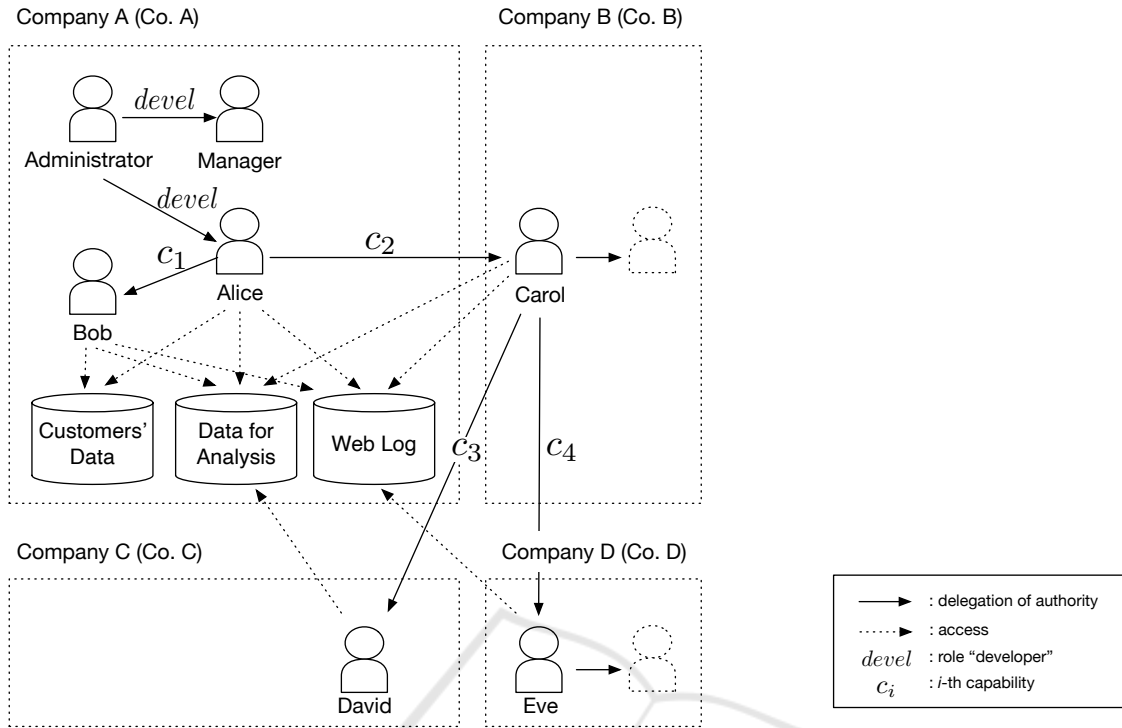
Figure 2: A scenario of collaborative development with multiple companies in dynamic environments.
