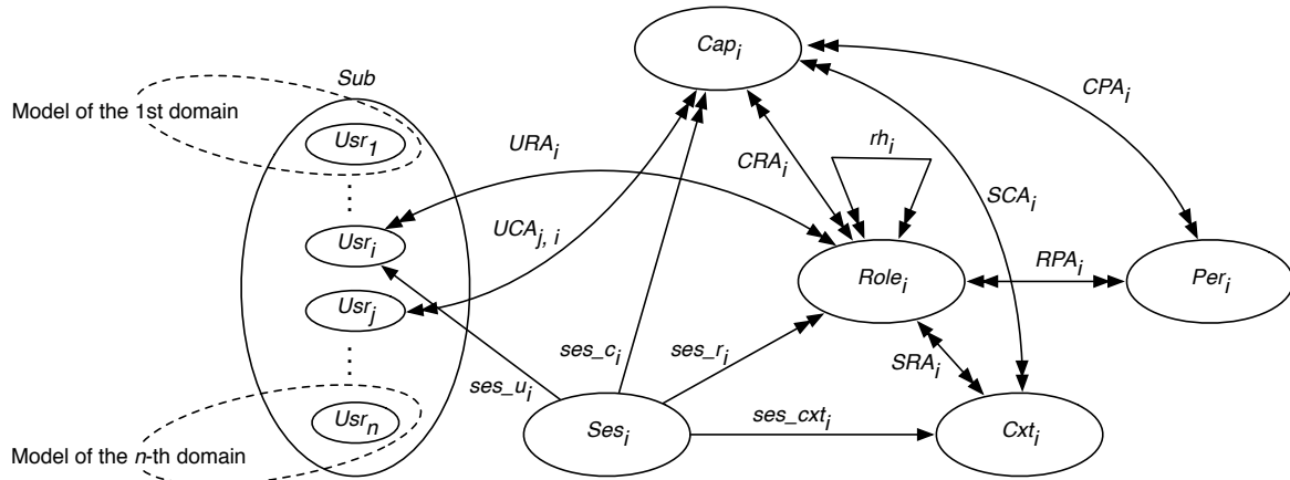
Figure 1: The family of C2RBAC models.
