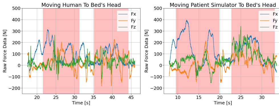
Figure 3: Raw force data (x, y and z axis) recorded while a nurse moves a human or a patient simulator towards the bed's headboard. The activity mainly consists of two turn movements (areas marked in red) which have been annotated using the data of a depth camera recording.
