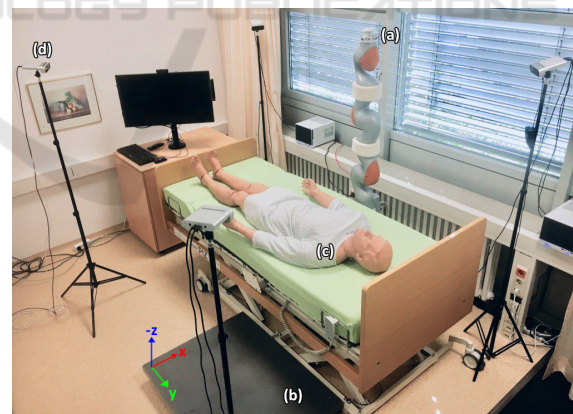
Figure 1: Setup for the support of nursing care bed activities using a bedside mounted KUKA LBR iiwa 7 R800 (a), an AMTI AccuPower portable force measuring platform (b), a rescue dummy functioning as a patient simulator with a weight of 80 kg (c) and a multi depth camera system (d).
