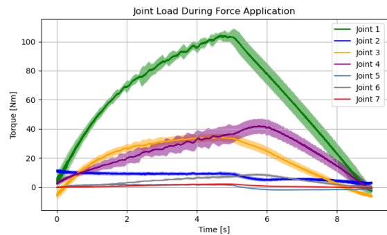
Figure 5: Visualization of the joint torques during the robotic load experiment where the robot applies a force to move the 80 kg weighing patient simulator. Mean torques of every joint and lower and upper error are visualized.
