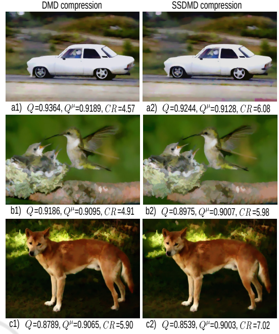
Figure 4: Comparison of DMD (a1–c1) with SSDMD (a2–c2) for three focus-and-context images. For each image, we show the standard MS-SSIM quality Q , spatial-saliency-aware MS-SSIM Q^\mu , and compression ratio CR .
