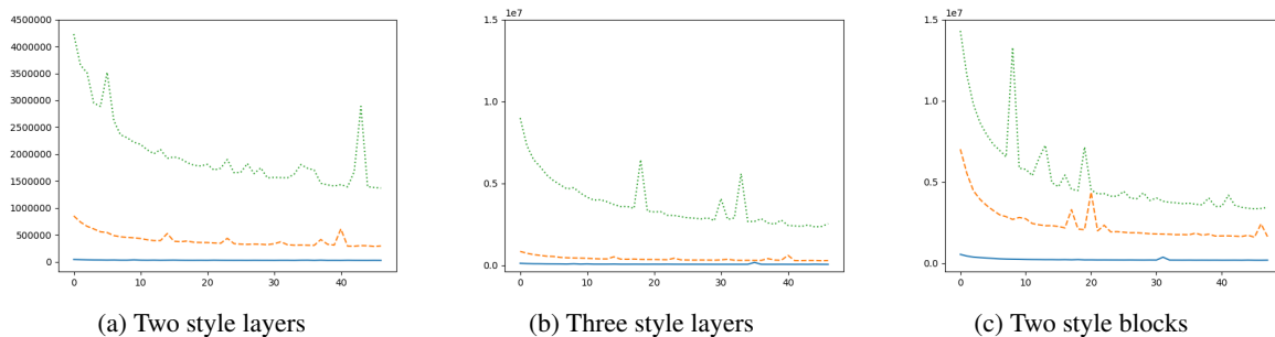
Figure 3: Style loss for each network with all loss coefficients = 2000 plotted against thousands of iterations. Continuous curve: fifth block layers, dashed curve: fourth block layers, dotted curve: third block layers.
