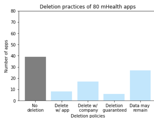
Figure 3: Deletion policies.
