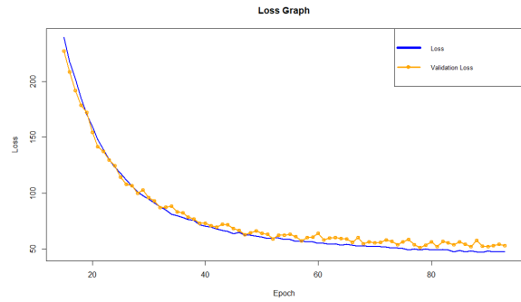
Figure 5: Training/validation loss in YOLO approach.
