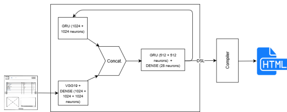
Figure 2: Hybrid approach architecture during inference.
