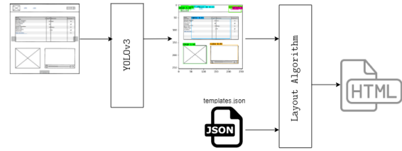
Figure 4: YOLO approach architecture during inference.
