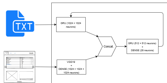
Figure 1: Hybrid approach architecture during training.
