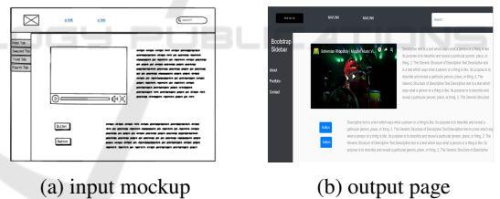
Figure 7: 2 nd example of prediction with YOLO approach.
