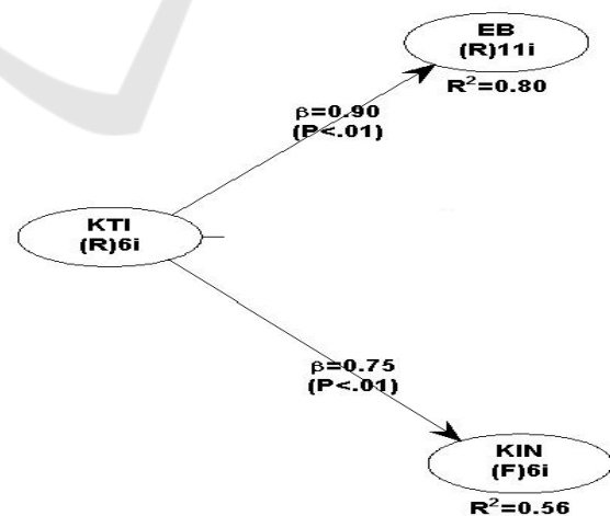
Figure 2 Output WarpPLS 5.0 Full Model
