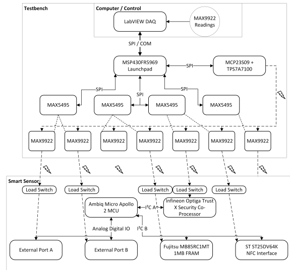
Figure 2: Design of Prototype B.
