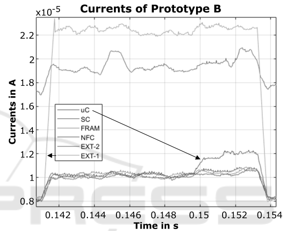
Figure 5: Current flow during measurements at Prototype B.
