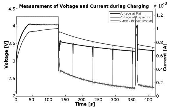
Figure 4: Measurement of the charging of Prototype A.
