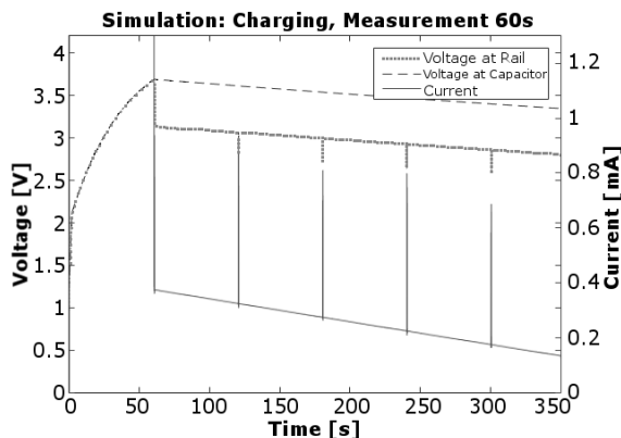
Figure 6: Simulation of the sensor charging.
