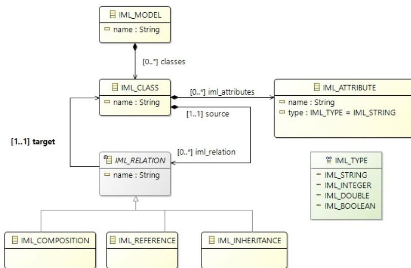
Figure 1: The IML Meta-Model implemented as an Ecore Model.
