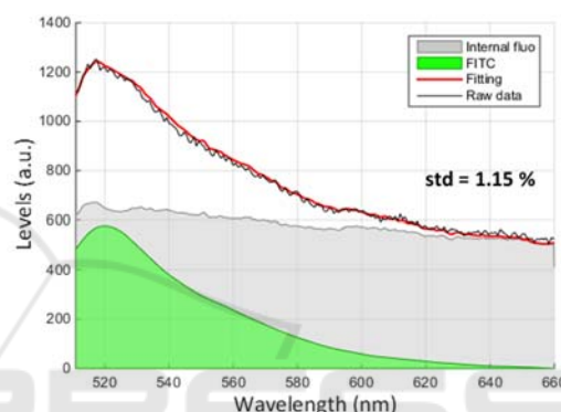
Figure 7: Extracting a weak FITC response using spectral fitting.
