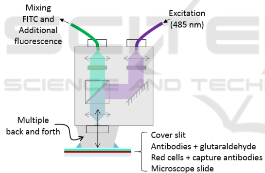
Figure 4: Origin of the additional fluorescence.
