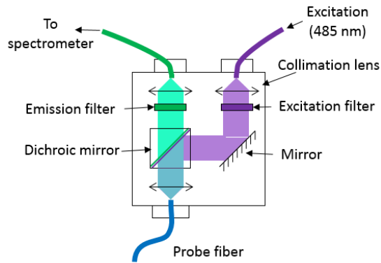
Figure 3: Fluorescence beam-splitter used in these experiments.
