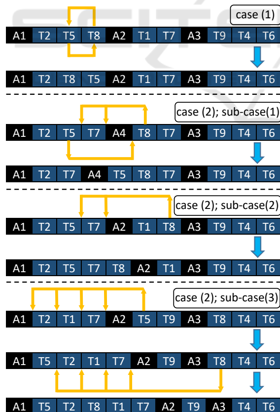
Figure 3: An example of the mechanism of PCR, showing both cases and all three possible sub-cases of case (2).
