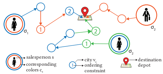
Figure 1: An Illustration of the ECTSP.
