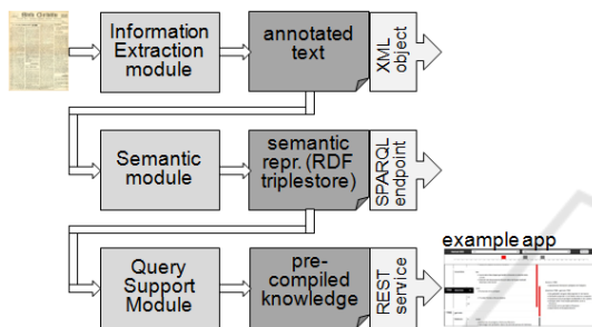
Figure 1: Pipeline architecture.
