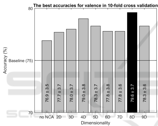
Figure 5: The best accuracy for valence with and without involving the NCA using kNN classifier in 10-fold cross validation after 1000 iterations and the baseline from (Ferdinando and Alasaarela, 2017) showed that the NCA enhanced the accuracies very well.
