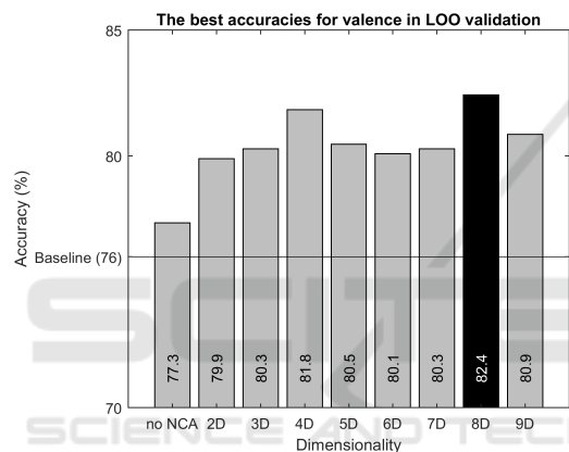
Figure 2: The best accuracy for valence with and without involving the NCA using kNN classifier in LOO validation and the baseline from (Ferdinando and Alasaarela, 2017) showed that the NCA improved the accuracies of system.
