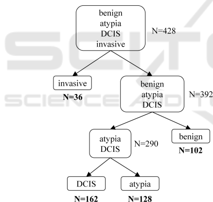
Figure 4: One-diagnosis-at-a-time classification.
