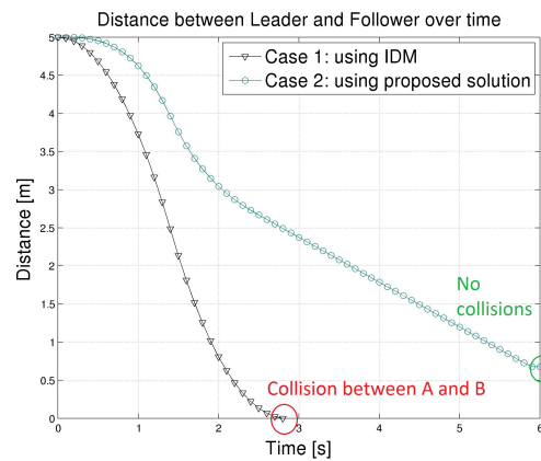
Figure 11: Inter-distance between vehicle A and B.
