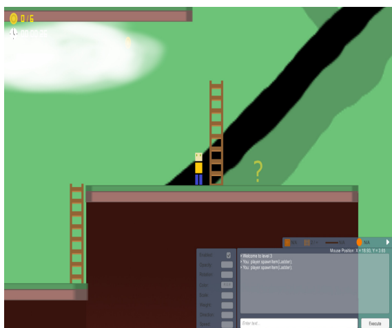
Figure 2: RunJumpCode Level 3.
