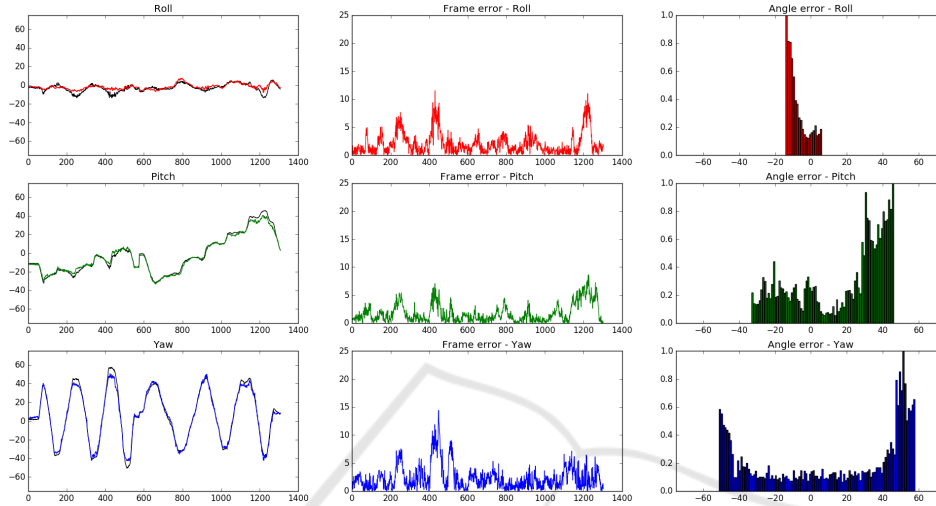
Figure 3: Experimental results on Biwi dataset : ground truth is black. The second column reports the angle error per frame, while the last column reports histograms that highlight the errors at specific angles.
