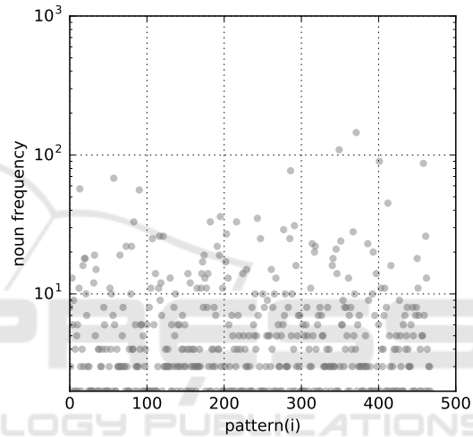
Figure 6: The frequency of nouns in an extraction pattern. The x-axis shows the number of extraction patterns found in our corpus (468). The y-axis shows the number of nouns grouped within that pattern.
