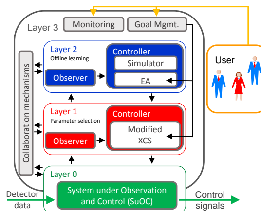
Figure 1: Architecture of an OTC-controlled TLC.
