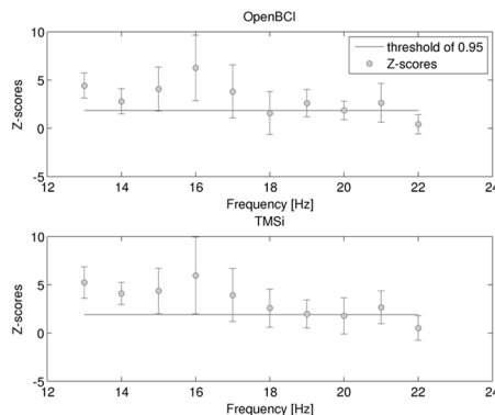
Figure 2: Z-scores for the differentiation of the SSVEP responses recorded by the OpenBCI (upper panel) and TMSi (lower panel) systems. The line indicates 5% significance of a correct determination of the target frequency by the BCI.
