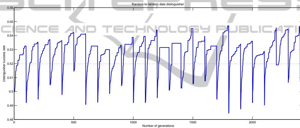
Figure 3: Example of success rate for distinguisher evolution between two sets of random data, the data set changed every 100 th generation (dotted line corresponds to average success of random guessing). Although no structure is present in data, the circuit is overlearning on a particular data set and thus exhibiting better success rate than random guess (increasing part of curve) before the test set is changed (a sudden drop in the success rate).
