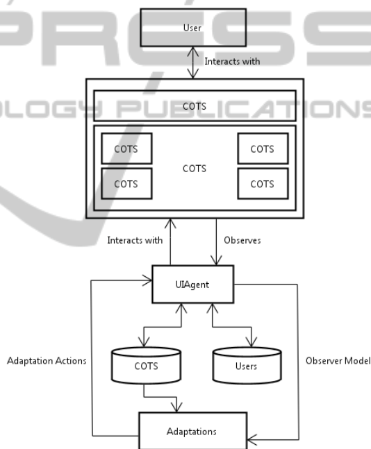
Figure 2: Interface Agent.
