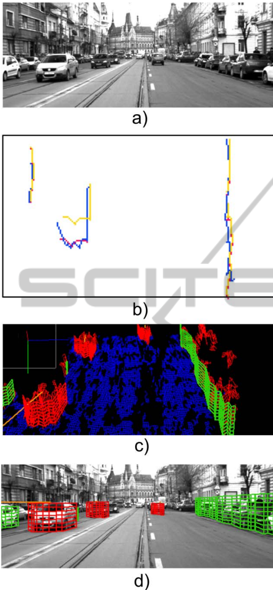
Figure 7: a) An urban traffic scenario. b) The alignment result (red color) between the model delimiter extracted in previous frame (yellow) and the data contour, extracted in the current frame (blue). c) The virtual view of the scene. The static obstacles are represented with green delimiters while the dynamic obstacles are colored with red. The speed vectors are associated to each dynamic entity. d) The representation result, projected on the left camera image.
