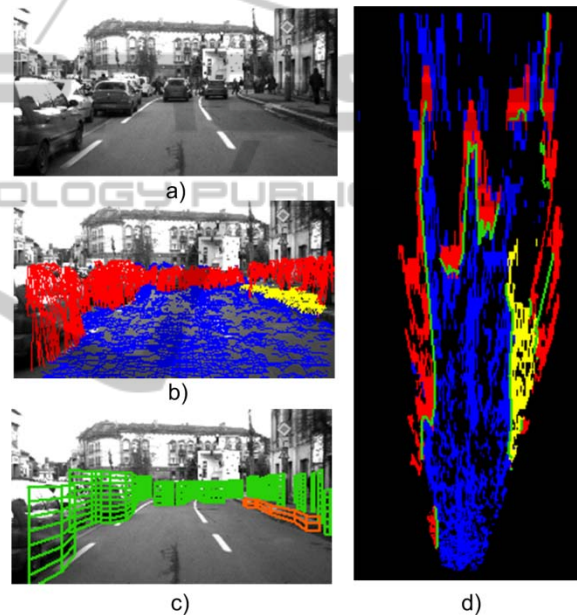
Figure 2: a) An urban traffic scene. b) The Elevation Map projected on the left camera image. d) The top view of the Elevation Map. The Elevation Map cells are classified (blue – road, yellow – traffic isle, red – obstacles). c) A compact representation of the environment. The extracted polygonal models are considered static. The extracted delimiters inherit the object information from the Elevation Map (green – obstacles, yellow – traffic isles).
