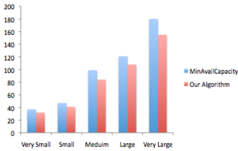
Figure 6: Number of initiated VMs.
