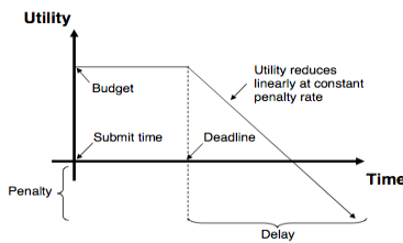
Figure 2: Penalty model.
