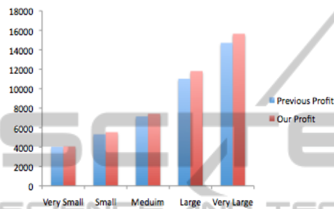
Figure 5: Provider profit.
