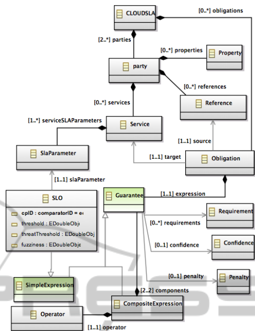
Figure 1: CSLA MetaModel.
