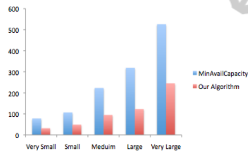
Figure 8: Penalty cost.
