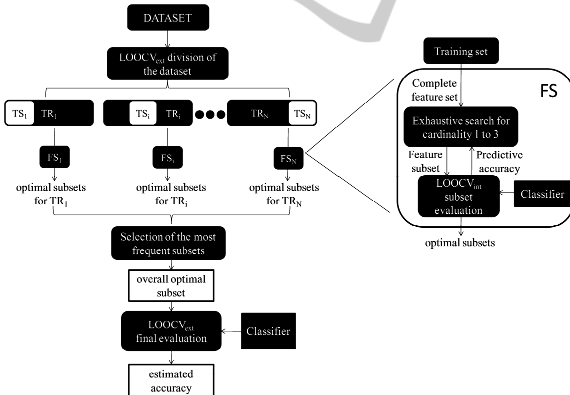
Figure 2: Feature selection procedure.
