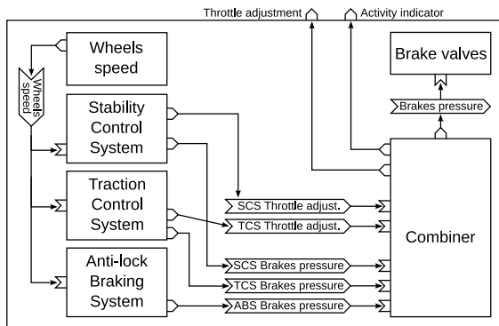
Figure 1: Component design of an electronic stability control (ESC) subsystem of a car.
