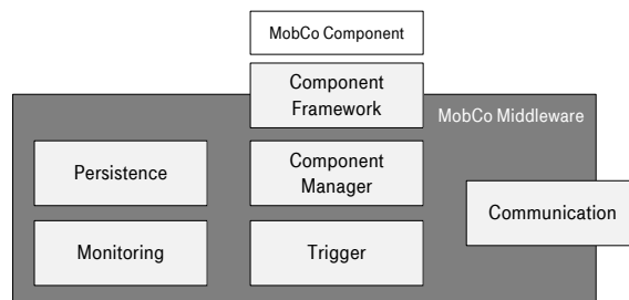
Figure 1: Subsystems of MobCo Middleware
