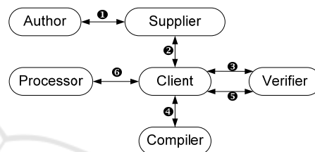
Figure 1: General WSbSC-RM.
