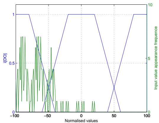
Figure 6: Membership functions and sampled measurements for DO.
