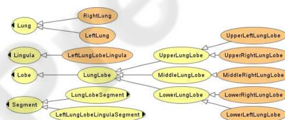
Figure 4: Lungs ontology - hierarchy of classes (created with OWLViz (Drummond, 2007)). Such a taxonomy of classes, related to each other through the specific properties defined in an ontology, allow the search engine to make intelligent (logical) decisions.
