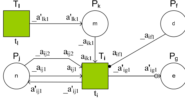
Fig. 5. mCRL2 actions mapped to the arcs and transitions of a Petri net.
