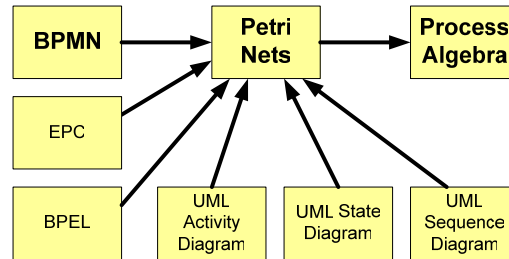
Fig. 1. Model transformations.
