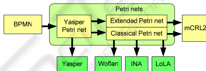
Fig. 4. Petri net analysis tools and related transformations.
