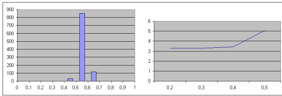
Figure 4: On the left, average distribution of users as regards Pearson coefficient. On the right, recall as threshold grows.
