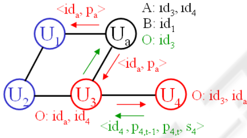
Figure 1: Exchanges of profiles p_x between peers U_x with different IDs.
