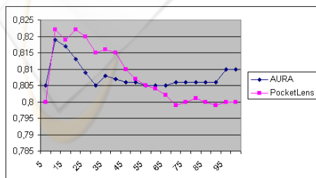
Figure 5: MAE as neighborhood size grows.
