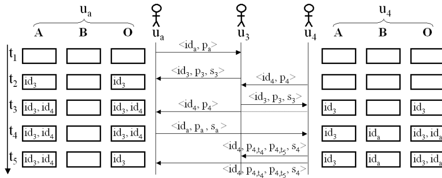
Figure 2: Example of user interactions.
