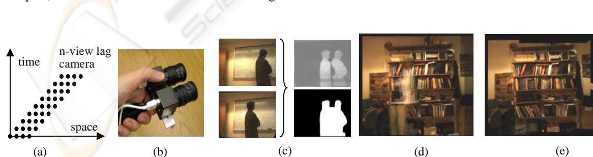
Figure 1: Lag Camera. (a) The general n-view lag camera samples a scene over space and time by ensuring at least one camera “lags” behind ( n=4 in figure). (b) A snapshot of our prototype 2-view lag camera. (c) Using images acquired from the same viewpoint but at two instances in time, we can easily identify foreground motion as well as acquire samples of the background in the presence of moving occluders. This allows us to capture busy, in-use environment despite temporary occluders appearing and disappearing from the images. Rendering results without (d) and with (e) our method are shown.
