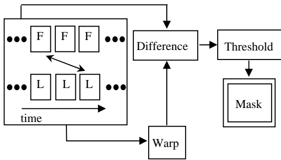
Figure 3: Computing Motion Masks. Each follow frame F is paired with a lead frame L. L is warped to the viewpoint of F. A difference image of frame F and Warp(L) is computed. The motion mask is generated by thresholding the difference image.
