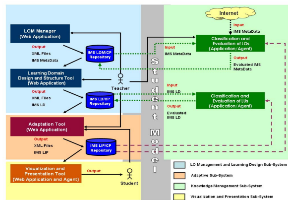
Figure 1: AHKME's structure.
