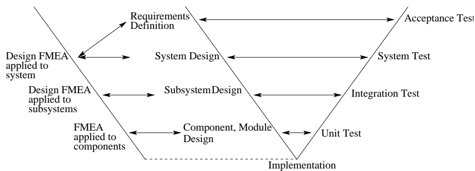
Figure 2: FMEA applied to the software system lifecycle.
