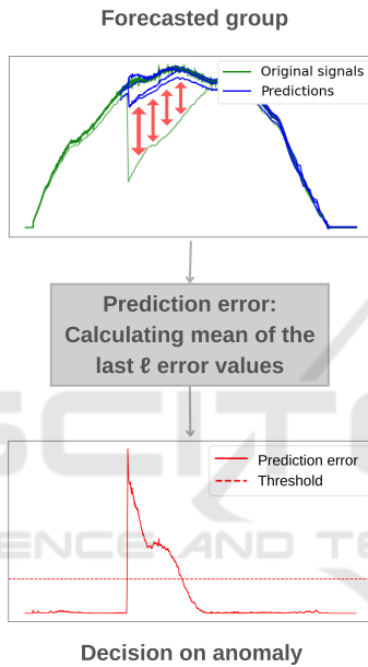
Figure 7: Visualization of the decision module.
