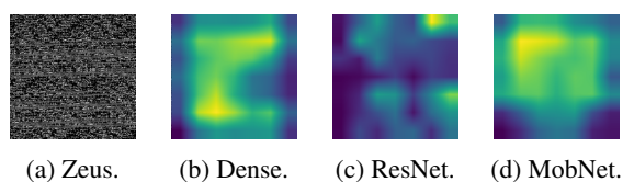
Figure 4: A plot of a malware sample which classified correctly belonging to Zeus including the heatmap of 3 models.
