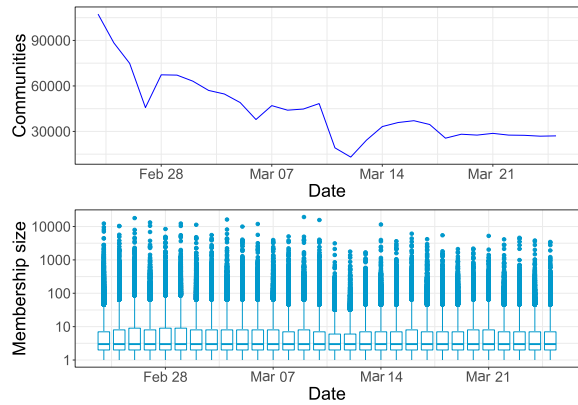
Figure 4: Daily community count and membership size.
