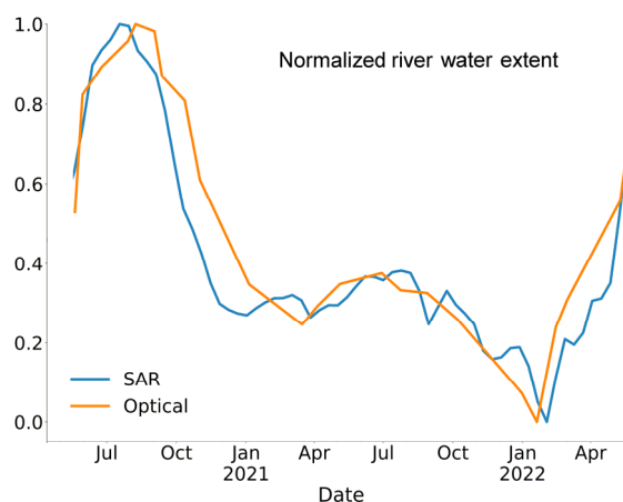
Figure 6: Normalized River Water Extent.
