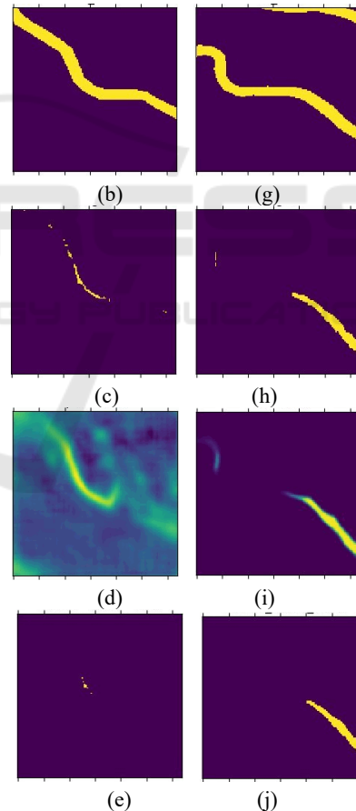
Figure 4: Samples after 100 training iterations (a-e), and after 30,000 training iterations (f-j); raw input (a,f); water surface mask (b,g); multispectral bands (c,h); raw output (d,i); discretized output (e,j).
