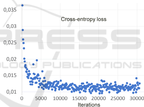
Figure 5: Cross-entropy loss against iterations.
