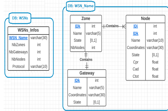
Figure 3: Entity relationship diagram for WSNs used by RWSNSim.
