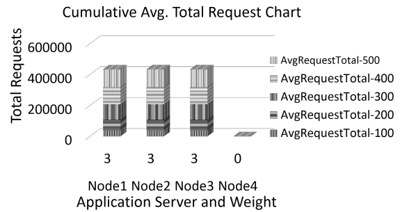
Figure 4: Overutilised VM.
