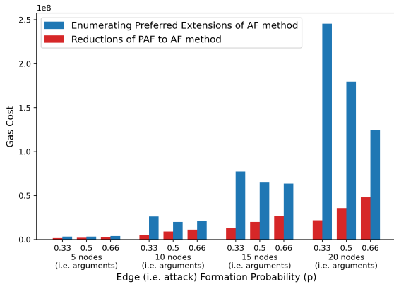
Figure 4: pafReductionToAfPr() and enumeratingPreferredExtensions() methods gas cost
