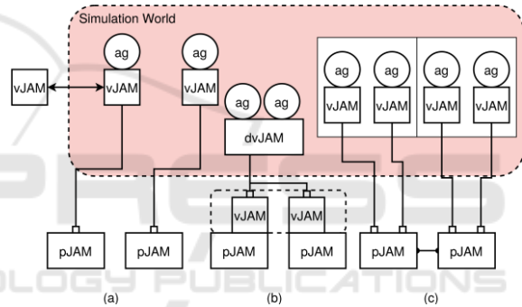
Figure 1: Distribution strategies: (a) Each virtual JAM node is assigned to a different physical node (b) A distributed virtual JAM node (dvJAM) is created by distributing agent processing on different physical nodes (c) in Regions of agents with their vJAM nodes are distributed on different pJAM nodes by preserving local context.
