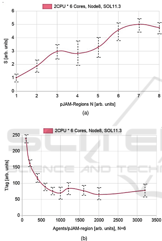
Figure 4: Results of the evaluation of the parallel traffic simulation. (a) Measured speed-up with respect to number of regions/pJAM nodes (b) Scaling of computation time with respect to agents/region with 6 pJAM regions (summarising all nodes and 10000 simulation steps).
