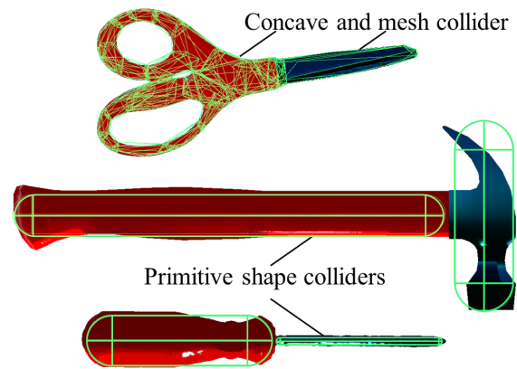
Figure 4: Geometry of the object colliders. Top: pair of scissors in closed fixed position with a concave collider applied to the handle (graspable side) and a mesh collider applied to its tool side. Middle and bottom: Hammer and screwdriver with two capsule colliders each; a capsule for the tool side and another one for the graspable side. All colliders are shown as green lines.
