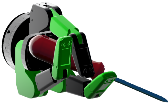
Figure 6: BarrettHand successfully grasping a screwdriver pointing away from the gripper.
