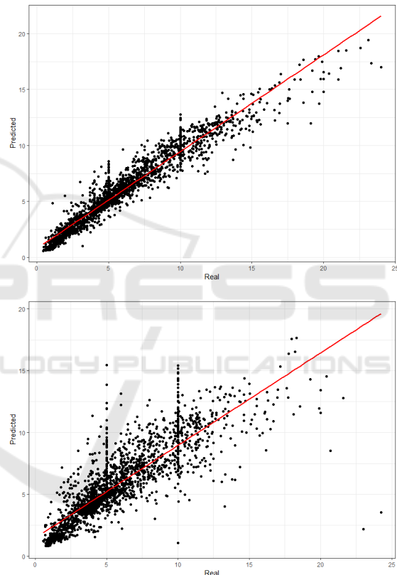
Figure 7: Regression Scatter Plot of Best Models for the Warp (Top) and Weft (Bottom) Tear Strength Predictions.
