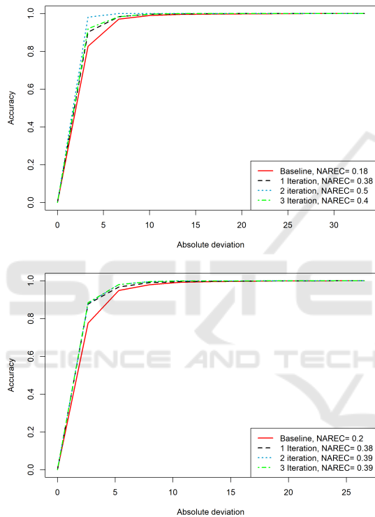
Figure 6: REC Curves for the Warp (Top) and Weft (Bottom) Tear Strength Prediction Models.
