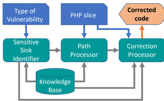
Figure 1: Automated Code Correction Approach Architecture.
