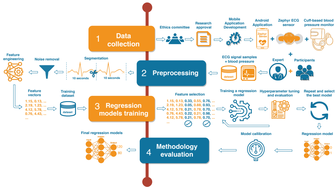
Figure 1: Methodology flowchart.
